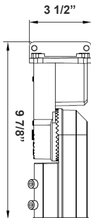
LFX-SF Slip Fitter 3 1/3" x 7 7/8" For 2-3/8" OD Pole/Pipe
